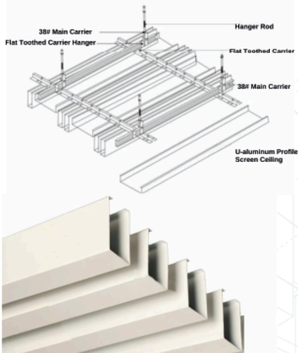
Installation Diagram For U-aluminum Profile Screen Ceiling
